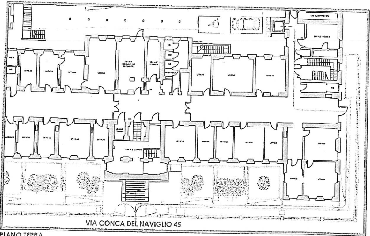
PIANO TERRA
