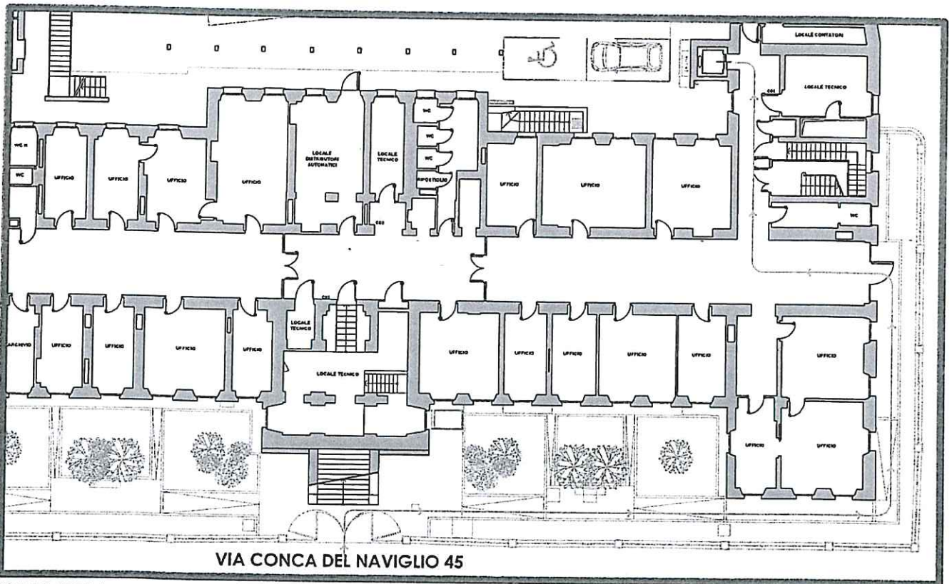
PIANO TERRA
